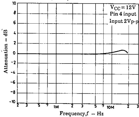
Frequency Characteristic
