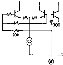
Expander Filter
