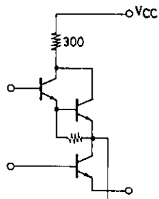
Expander Output
