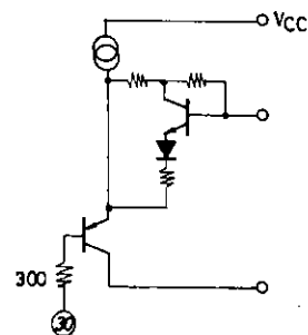
Volume Contr.
