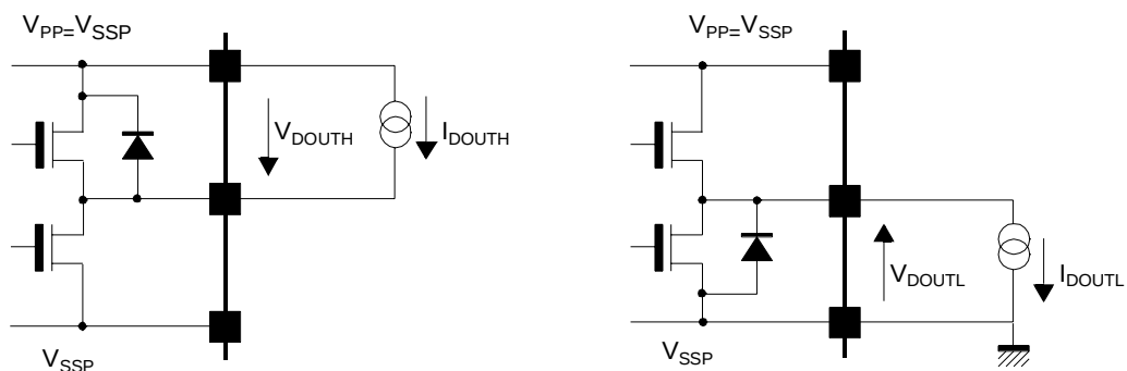
Figure 2: Test Configuration
