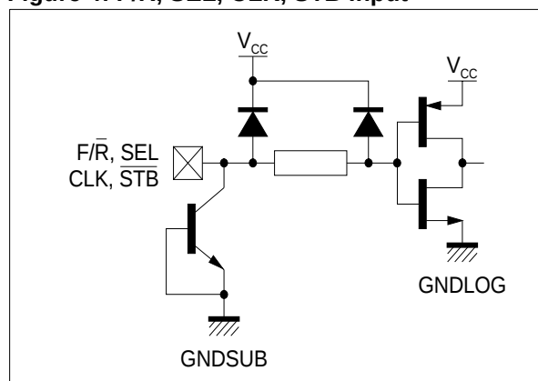
Figure 4: \overline{\text{F/R}} , \overline{\text{SEL}} , CLK, \overline{\text{STB}} Input
