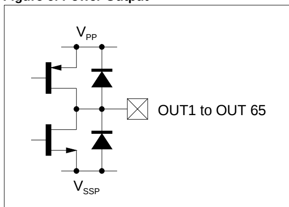
Figure 6: Power Output
