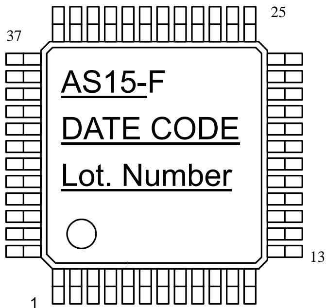
LEAD FREE TQFP48 ( MAKING )
