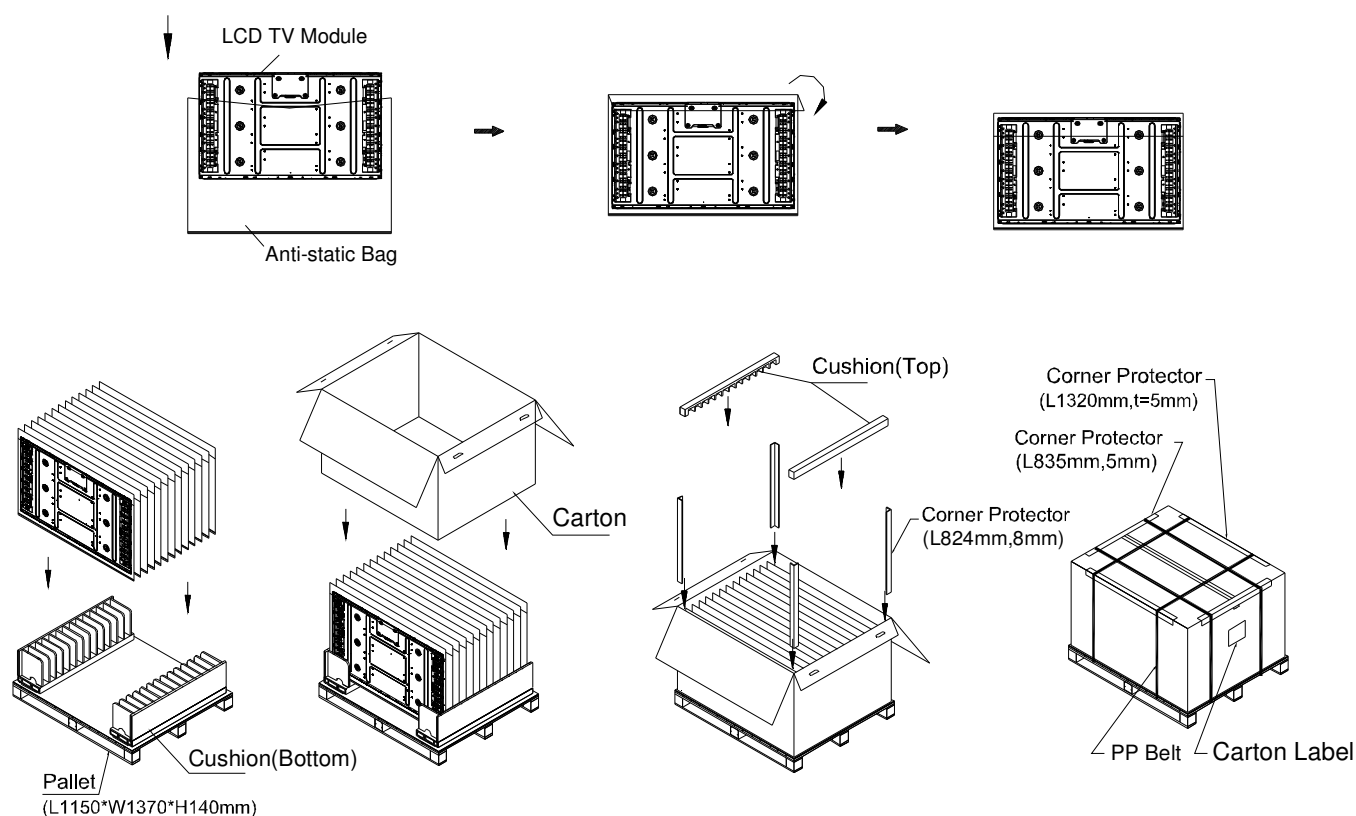
Figure. 9-3 Packing method
