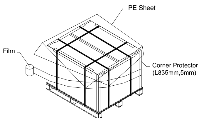
Figure. 9-4 Packing method
