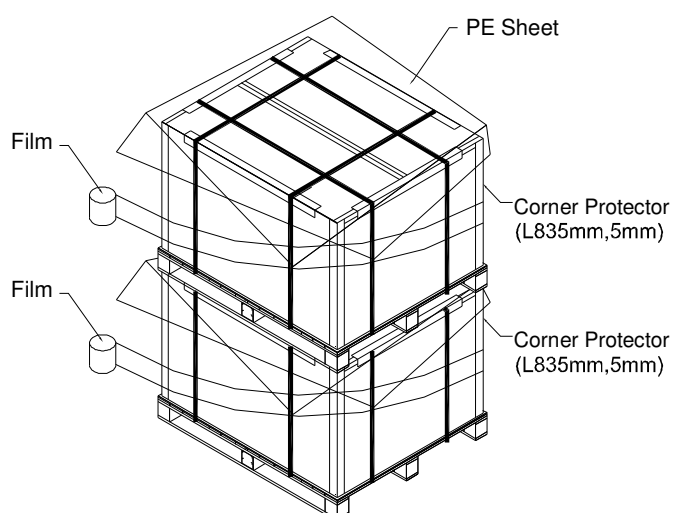
Figure. 9-4 Packing method
